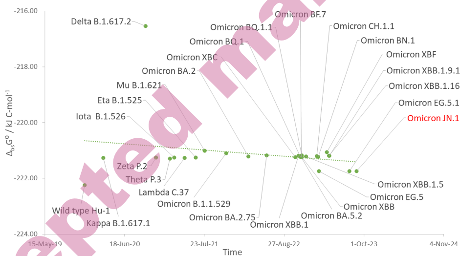
Fig 2. Gibbs energies of biosynthesis of different SARS-CoV-2 variants during the time evolution of the virus. \Delta_{bs}G^\theta represents standard Gibbs energy of biosynthesis.
