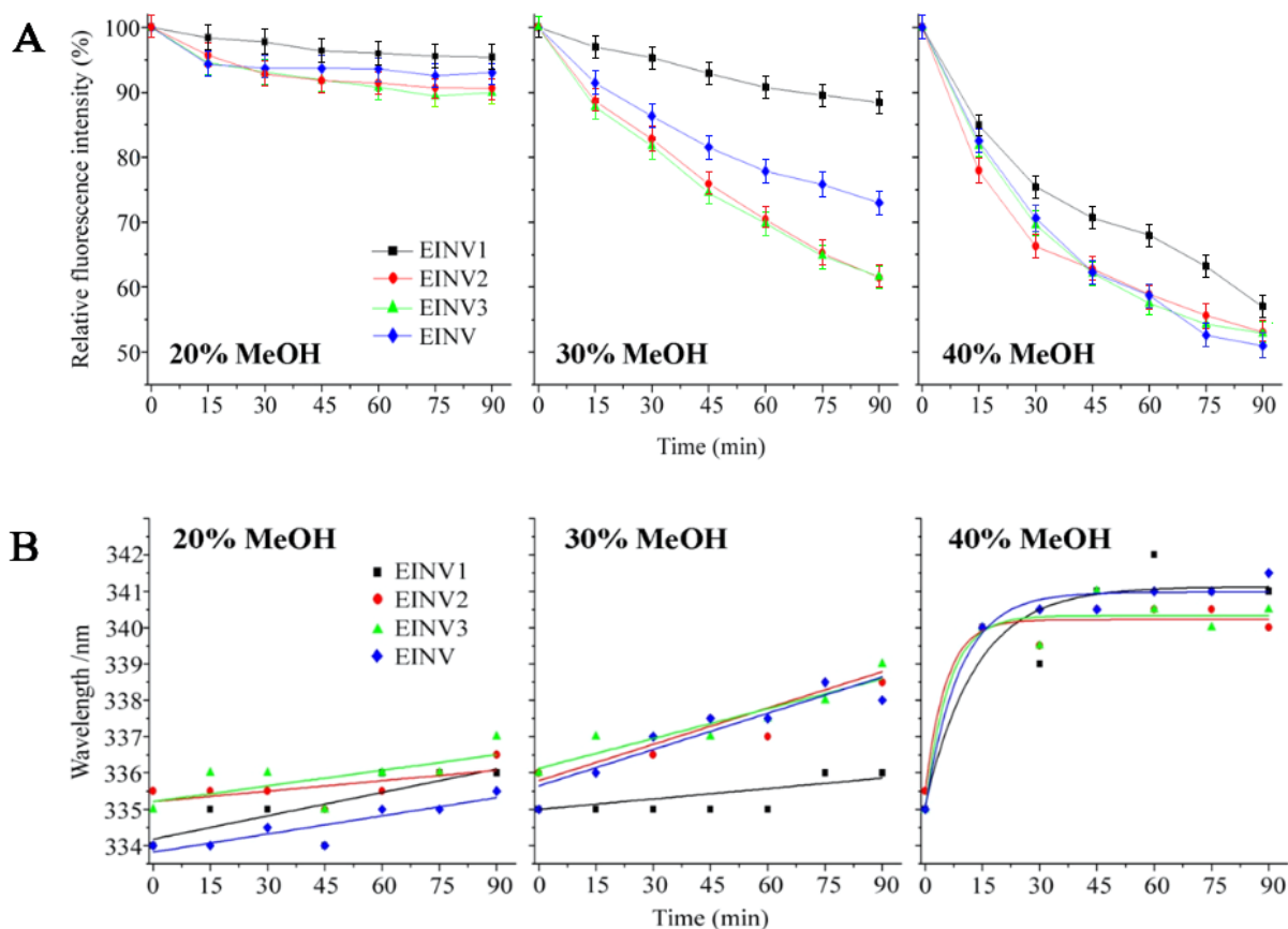
Fig. 3: Effect of different concentrations of methanol on external invertase glycoforms (EINV1–EINV3) and total external invertase (EINV) as monitored by fluorescent spectroscopy. Different concentrations (v/v) of methanol in 50 mM acetate buffer pH 5.0 at 40°C. (a) The change of intensity of intrinsic fluorescence at 340 nm. (b) The wavelength shift of the fluorescence emission maximum.
