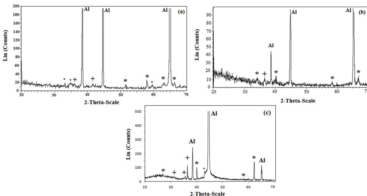
Figure 5. Diffraction patterns of aluminium sample after: a) 1, b) 2 and c) 5 h of magnesium underpotential deposition at E_x = 60 mV vs. Mg/Mg(II) in non-aqueous eutectic mixture \text{Mg}(\text{NO}_3)_2 + \text{NH}_4\text{NO}_3 at T = 460 K; a) (•) (hcp) - \text{Al}_{0.9}\text{Mg}_{3.1} [32]; (*) (bcc) - \text{Al}_{12}\text{Mg}_{17} [33]; (+) (hcp) - \text{Mg}_2\text{Al}_3 [34]; b) (+) (hcp) - \text{Mg}_2\text{Al}_3 [34]; (*) (bcc) - \text{Al}_{12}\text{Mg}_{17} [33]; c) (+) (hcp) - \text{Mg}_2\text{Al}_3 [34]; (*) (bcc) - \text{Al}_{12}\text{Mg}_{17} [33]; (•) - (rhombohedral) \text{MgO}_4 [35].
