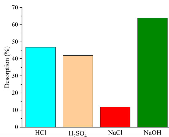
Figure 12. Desorption of CIP from H_Co/C-S using different eluents.
