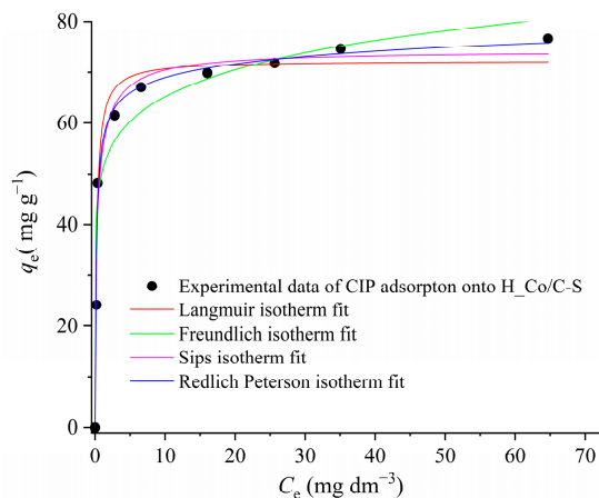
Figure 9. Adsorption isotherms for CIP adsorption onto H 2 Co/C-S ( m_{ads} = 10 mg; C_{CIP} = (5–80) mg g -1 , V = 50 mL; t = 1440 min; T = 25 °C; pH 5.1).
