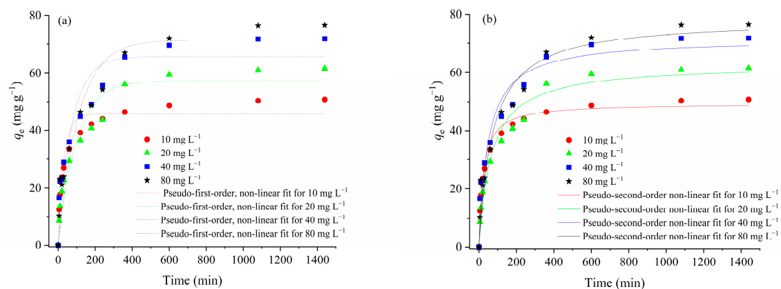
Figure 8. Non-linear plots of experimental data for CIP adsorption onto H_Co/C-S by (a) the pseudo-first-order kinetic model, and (b) the pseudo-second-order kinetic model.
