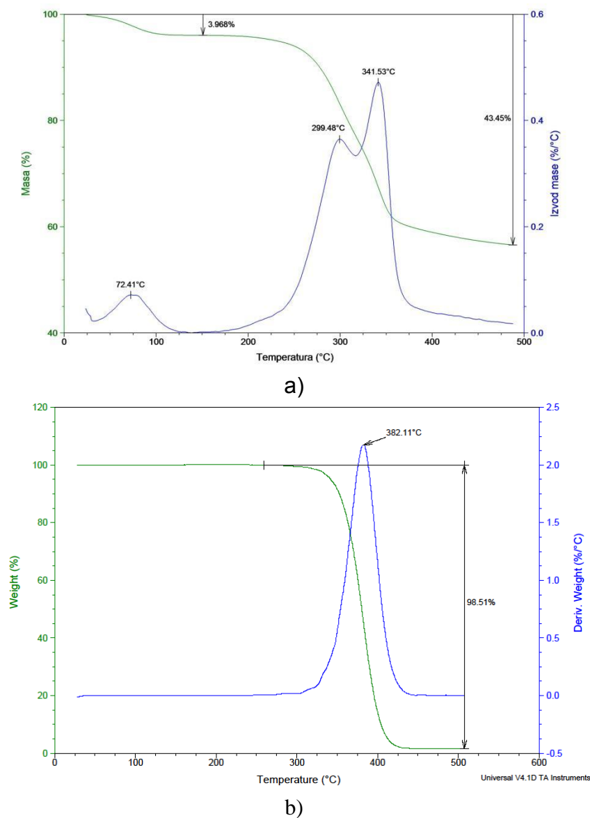
Figure 1. The results of thermogravimetric analysis of composites a) lignocellulose matrix filled with copper powder, treatment pressure of 20 MPa; b) PMMA matrix filled with copper powder.
