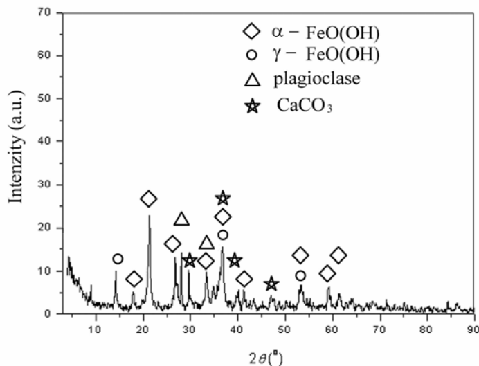
Fig. 3. XRD diagram of the corrosion products of the spearhead
