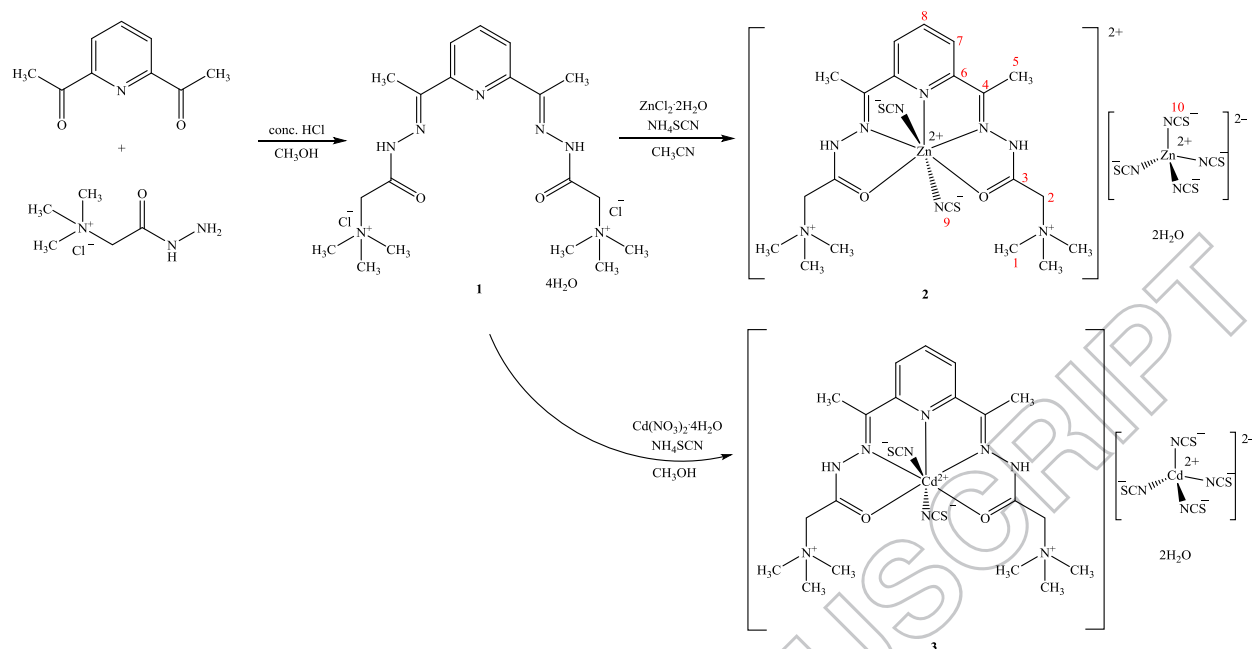
Scheme 1. Synthesis of ligand ( H 2 LC 2 ), Zn(II) ( 1 ) and Cd(II) ( 2 ).
