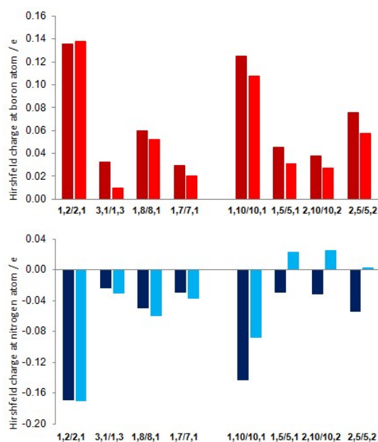
Figure 3. Hirshfeld charges at boron atom (upper part) and nitrogen atom (lower part) in eight orientational isomers of BN naphthalenes: dark red/dark blue colour represents charges in the more stable of the two isomers.
