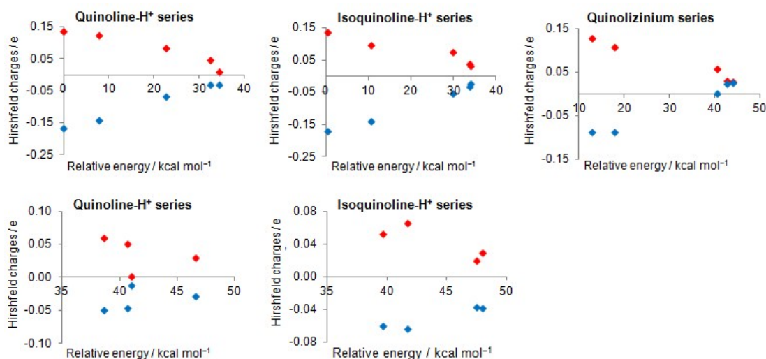
Figure 5. Hirshfeld charges at boron atom (red colour) and nitrogen atom (blue colour) in BN naphthalenes derived from quinoline- H^+ , isoquinoline- H^+ and quinolizinium cation. Upper part: isomers having heteroatoms in one ring. Lower part: isomers having heteroatoms in separate rings.
