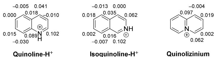
Figure 4. Hirshfeld partial atomic charges in protonated quinoline and isoquinoline, and quinolizinium cation.
