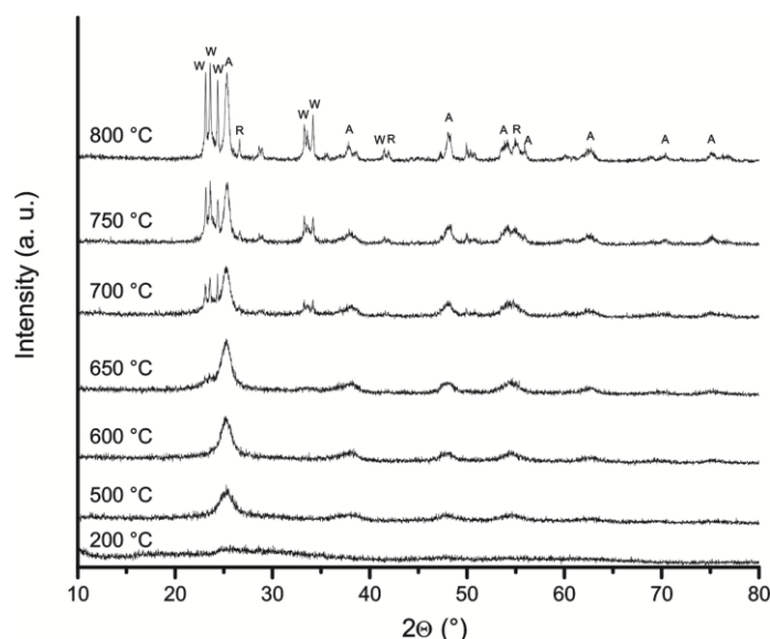
Fig. 1. XRD patterns of \text{WO}_x\text{-TiO}_2 powders for different sintering temperatures (A: anatase, R: rutile, W: tungsten oxide).
