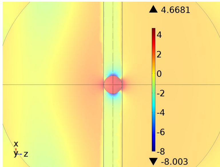
Fig. 10 Field enhancement around ITO nanoparticle for infrared detector enhancement, calculated by FEM simulation. Light is incident from right. r=60 nm, \lambda_p=625 nm, \lambda =2.6 \mu\text{m} , permittivity of the dielectric layer is 8
