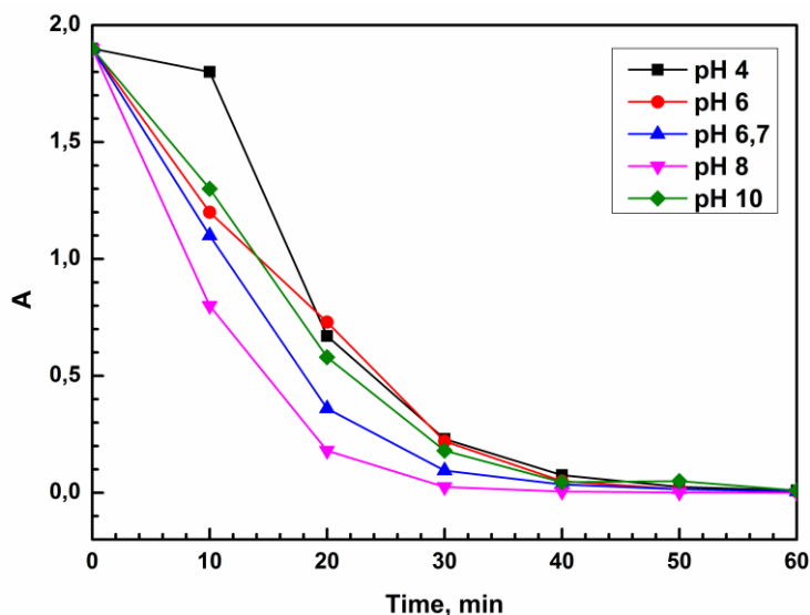
Figure 7. Decolorization as function of pH for Reactive Blue 52, 200 ppm solution
