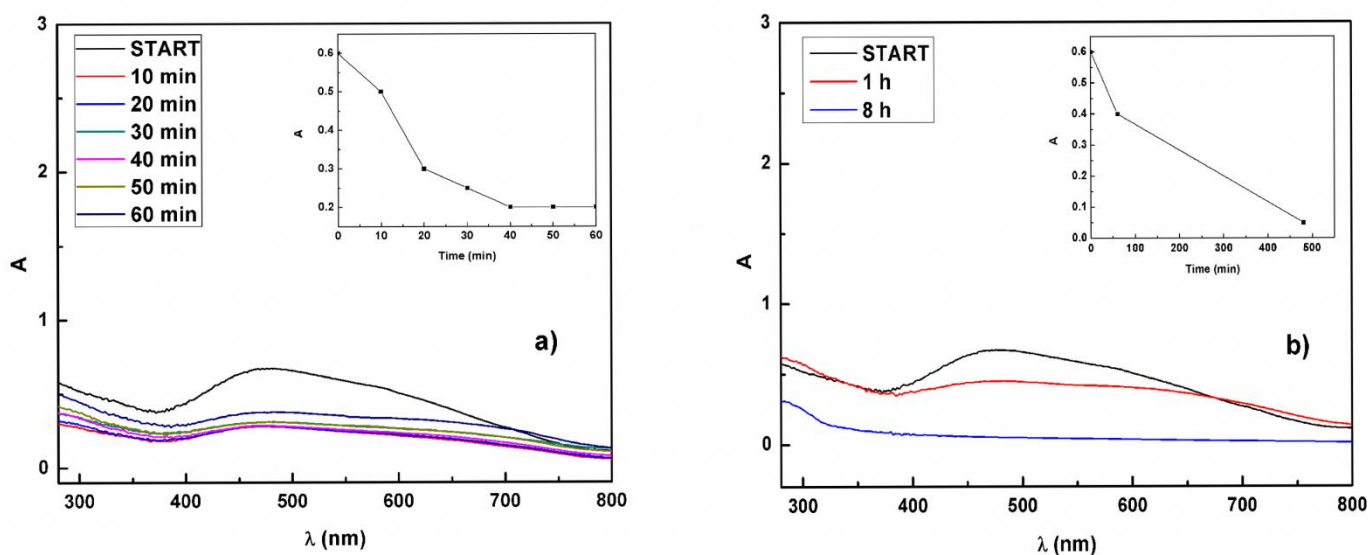
Figure 4. Absorption spectra of Reactive Black 5: a) with membrane, b) without membrane, Inset plot: Decrease of absorbance with time at \lambda_{\text{max}} = 590 nm
