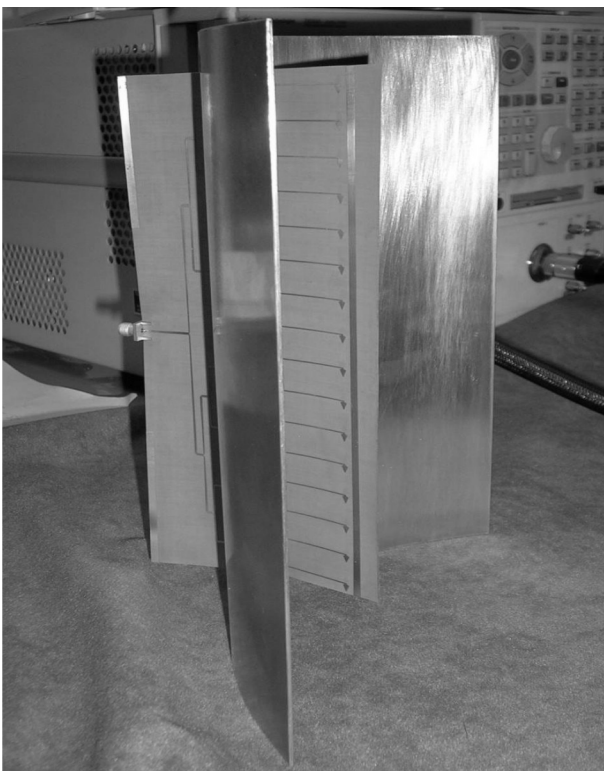
Figure 8: Photograph of the realized 23 GHz antenna array (C) in the cylindrical-parabolic reflector with uniform feed distribution.
