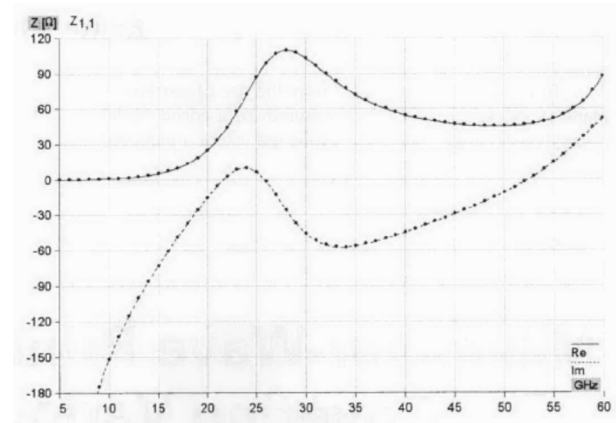
Figure 2: Real and imaginary parts of the pentagonal dipole impedance* as a function of frequency ( \epsilon_r=2.1 , h=0.254 mm, S^{**}=\lambda/4 ).
