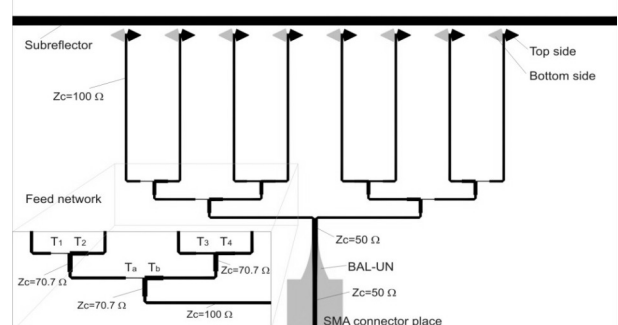
Figure 5: Example of feed network with impedance transformers ( T_{1-4} , T_{a-b} ) for tapered distribution (detail in the left lower corner).
