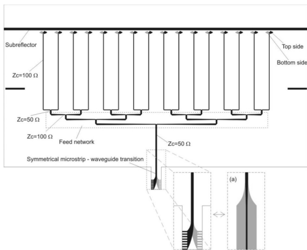
Figure 3: Printed antenna array with the subreflector and the feed network integrated on the same dielectric substrate.
