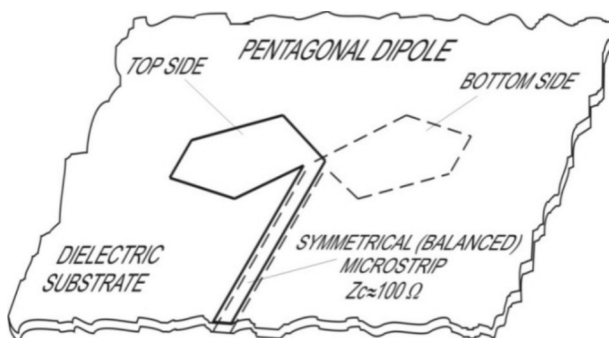
Figure 1: Printed pentagonal dipole as a basic element of the antenna array.
