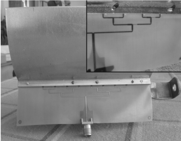
Figure 7: Photograph of the realized 26 GHz antenna array (B) in the cylindrical-parabolic reflector with tapered feed distribution with the detail of the tapered feed network.
