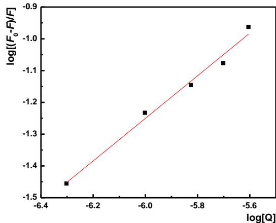
Figure S6. Log-log plot for the determination of binding constants K_b , and the number of binding sites n for binding of 16 to HSA ( c=5 \times 10^{-7} M) T=298 K; pH = 7.34; \lambda=323 nm; linear equation: y=2.77+0.67x (For the calculation of binding constants, only points within linear dependence were used (1-5 molar equivalents).)
