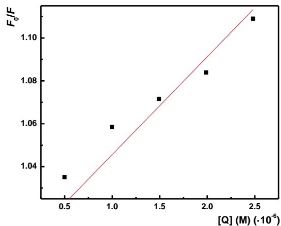
Figure S5. The Stern-Volmer plot for binding of 16 to HSA ( c=5 \times 10^{-7} M), T=298 K; pH = 7.34; \lambda=323 nm; linear equation: y=1+45628.8x (For the calculation of binding constants, only points within linear dependence were used (1-5 molar equivalents).)
