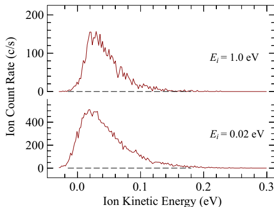
Fig. 3 Ion kinetic energy distributions recorded at the two incident electron energies indicated.
