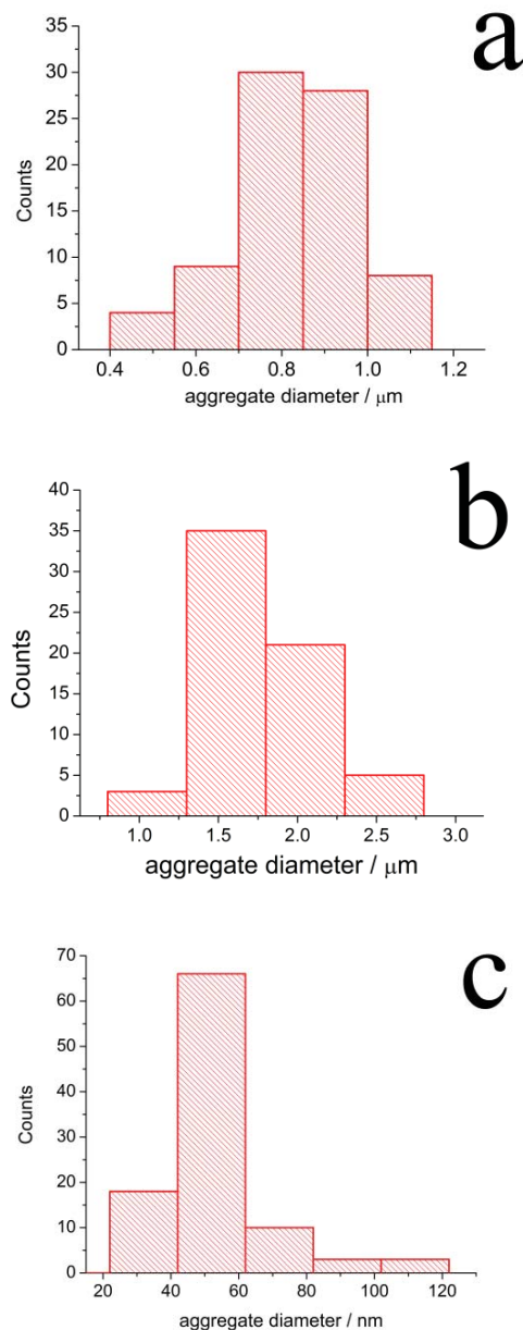
Figure 6. Aggregate size (AFM data) distribution of the Zn-Mn coatings electrodeposited from DES 1:1 at a) 3 and b) 20 \text{ mA cm}^{-2} , and from DES 3:1 at c) 3 \text{ mA cm}^{-2} .
