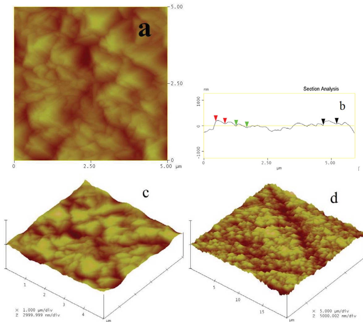
Figure 1. a) 2D; b) cross section height profile analysis; and 3D AFM images of the scanned area of: c) 25 \mu\text{m}^2 and d) 400 \mu\text{m}^2 of the Zn-Mn films deposited from DES 1:1 at 3 \text{mA cm}^{-2}
