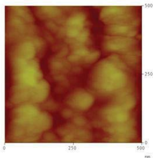
Figure 5. 2D AFM image of the scanned area of 0.25 \mu\text{m}^2 of the Zn-Mn film deposited from DES 3:1 at 20 \text{ mA cm}^{-2}
