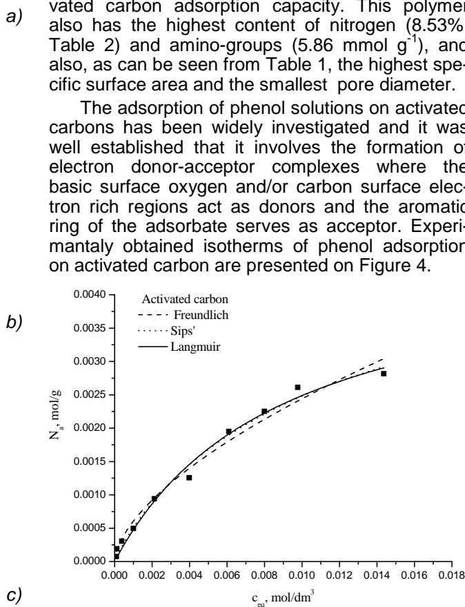
Figure 4 - The isotherms of phenol adsorption on activated carbon
